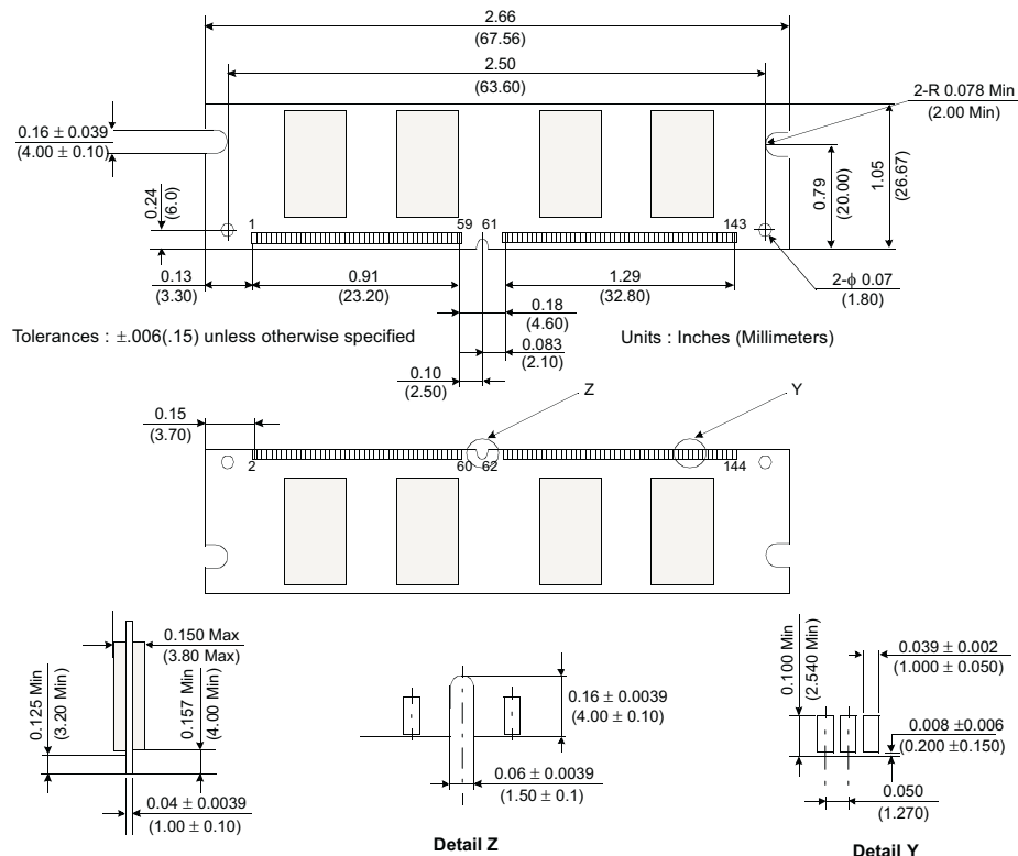
Figure 1: KVR133X64SC3L/128 144-Pin SDRAM Module
