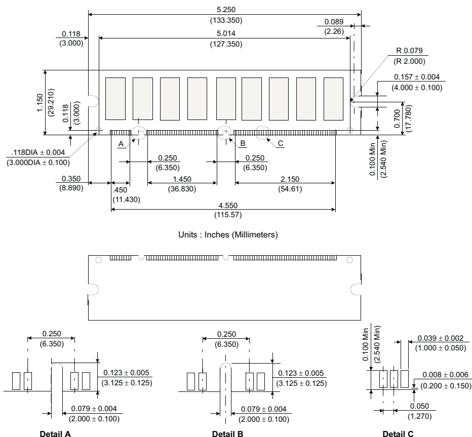
Figure 1: KVR133X72C3/256 168-Pin SDRAM Module
