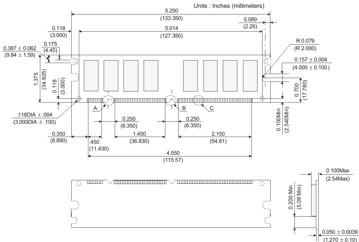
Figure 1: KVR100X64C2/64 168-Pin SDRAM Module
