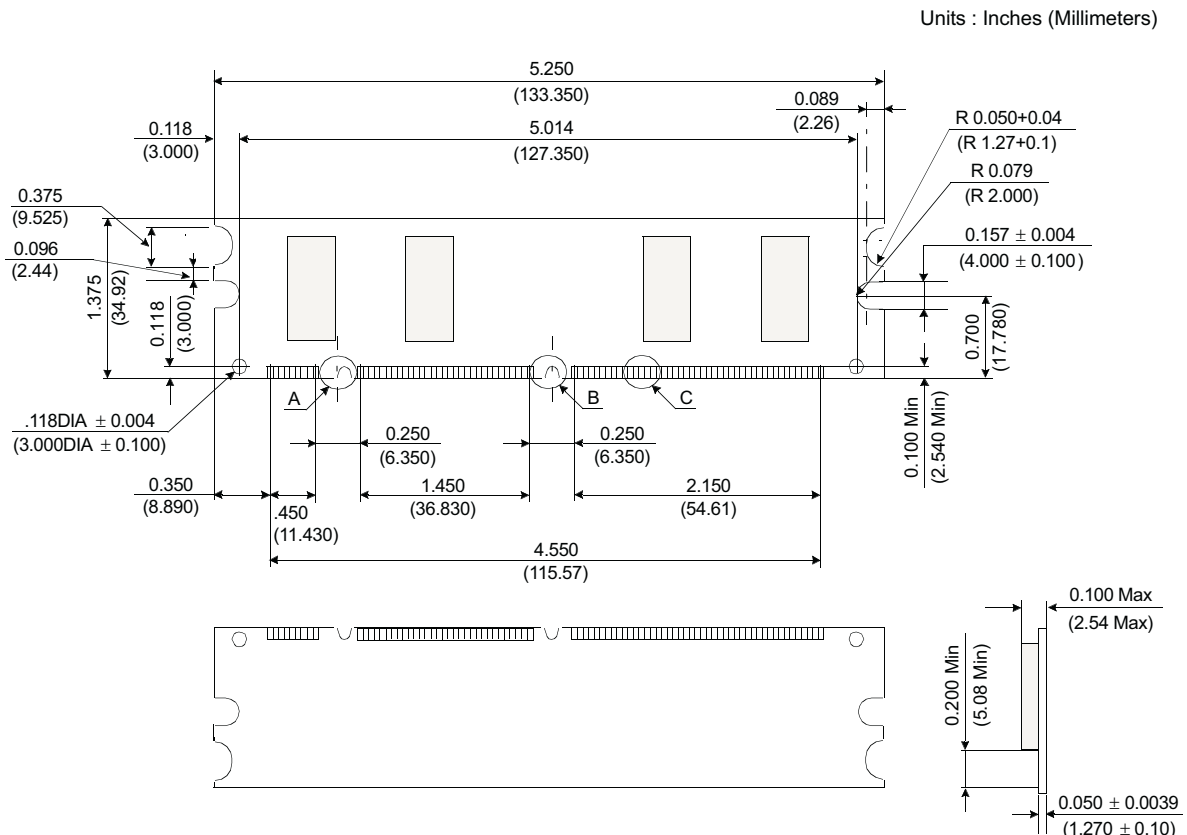
Figure 1: KVR133X64C3SS/128 168-Pin SDRAM Module
