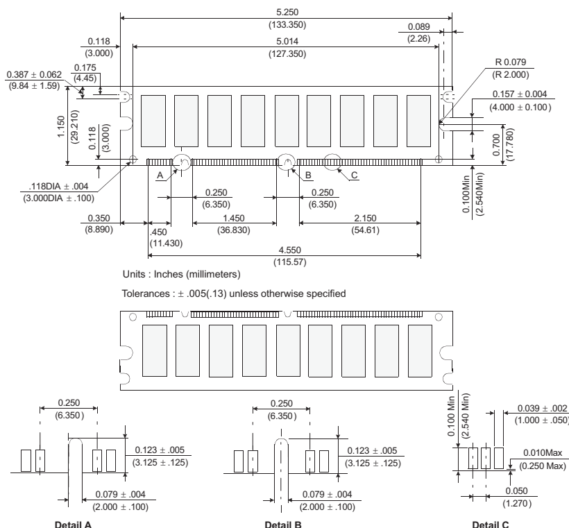
Figure 1: KVR100X72C2L/128 168-Pin SDRAM Module
