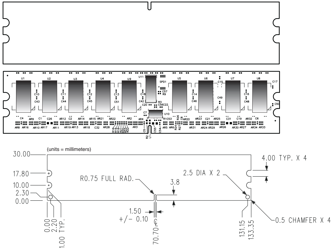
Figure 1: KVR400D2R3/256 240-Pin DIMM
