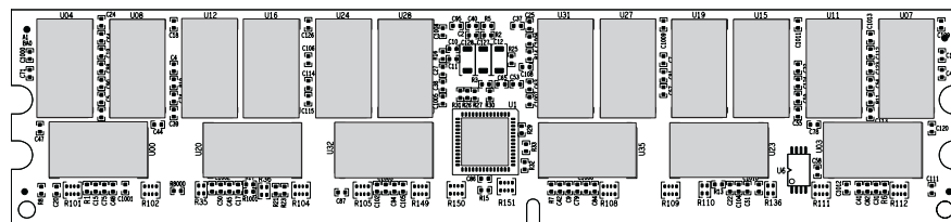
PRIMARY SIDE
