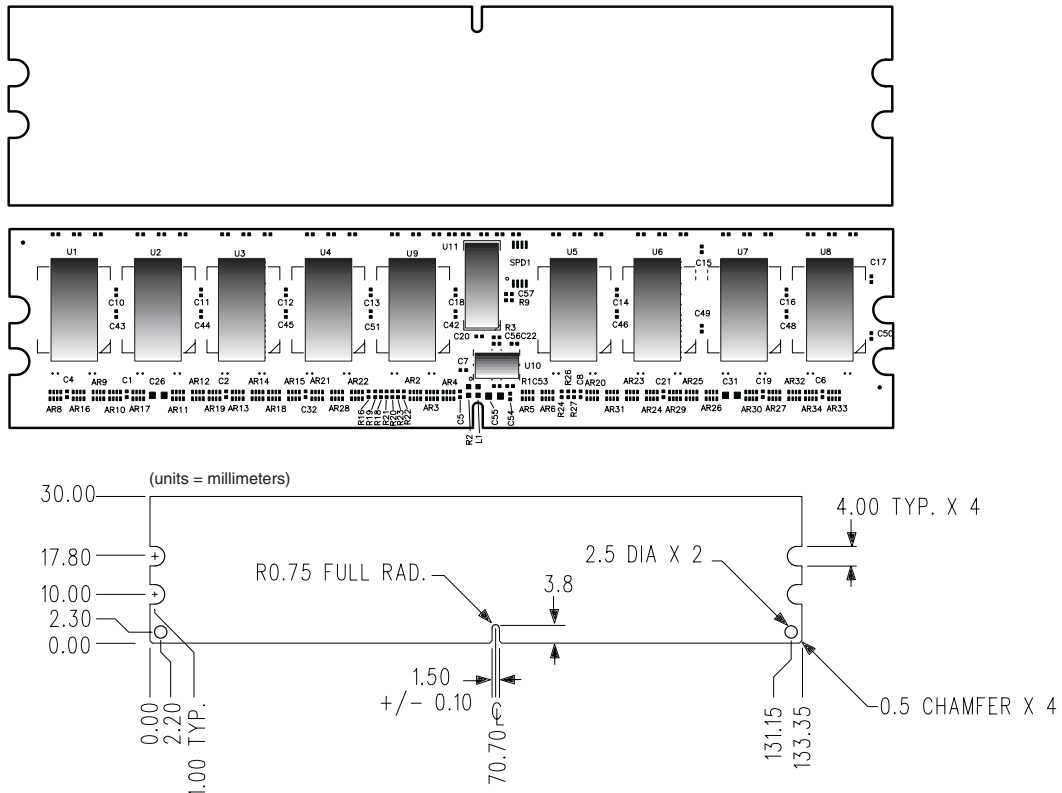
Figure 1: KVR400D2S8R3K2/1G 240-Pin DIMM
