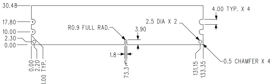
Figure 1: KVR333D4R25/1G 184-Pin DIMM
