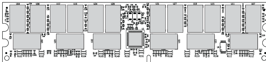
PRIMARY SIDE
