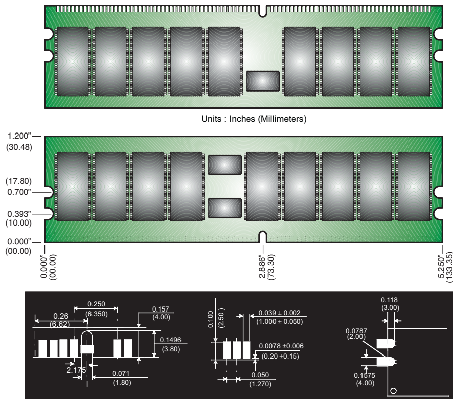
Figure 1: KVR400D8R3A/1G 184-Pin DIMM
