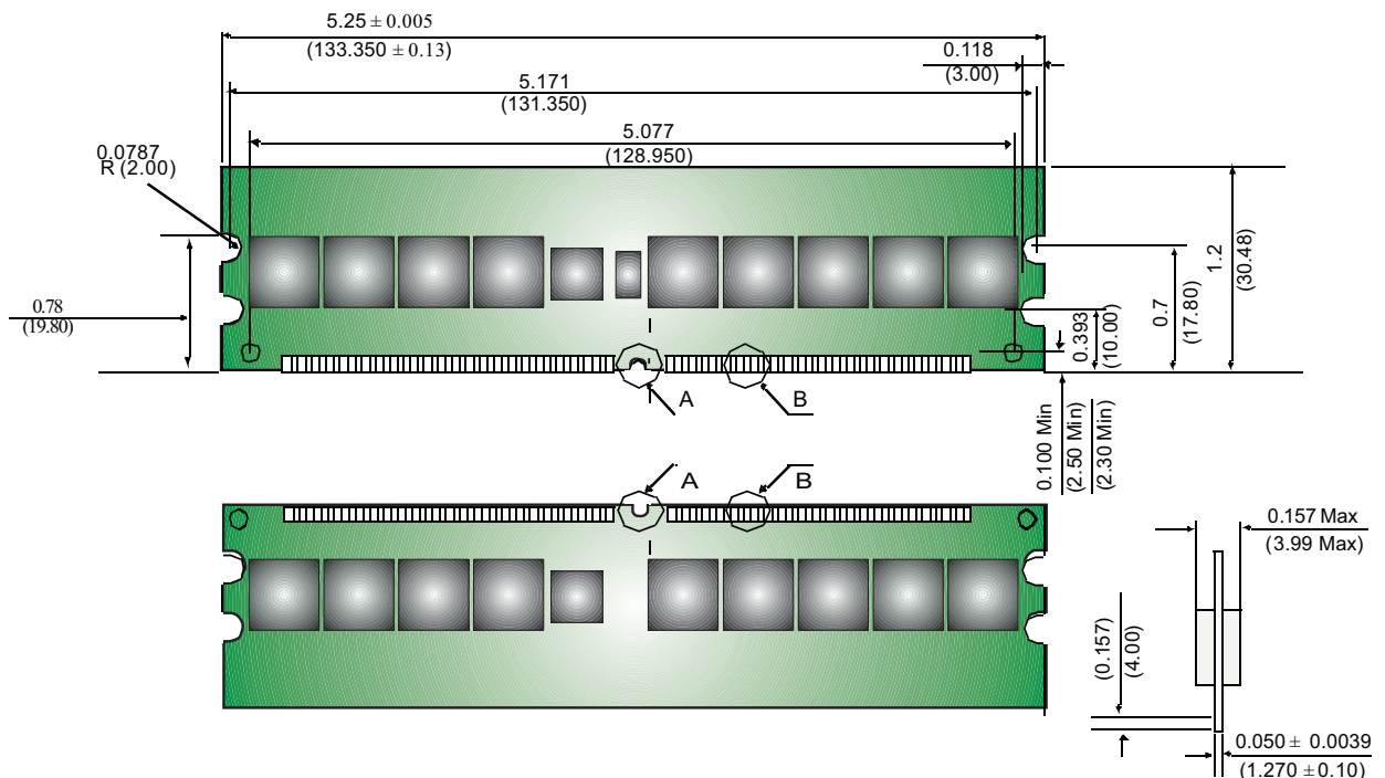
Figure 1: KVR400S4R3AK2/1G 184-Pin DIMM
