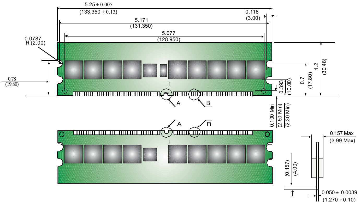
Figure 1: KVR333S4R25/1G 184-Pin DIMM
