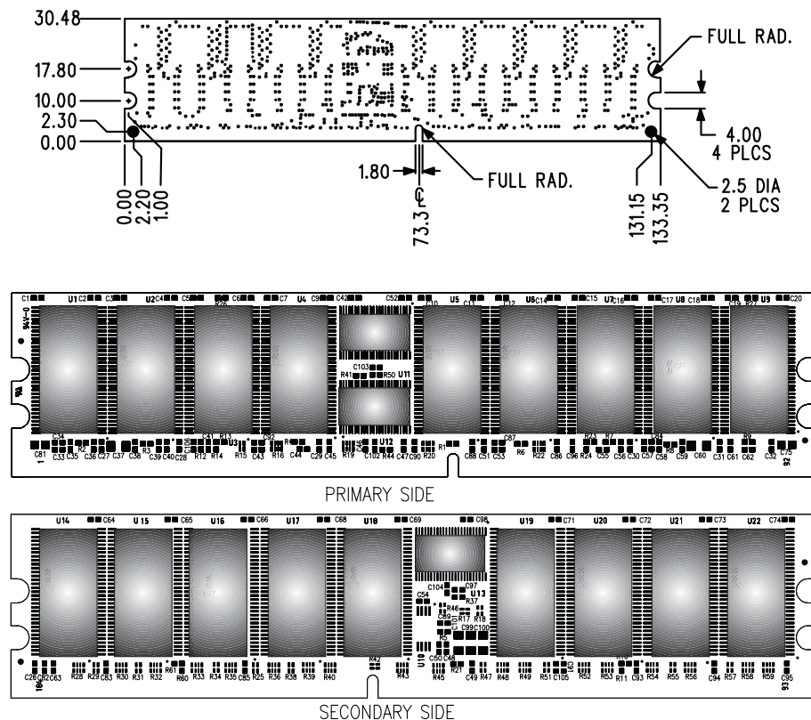
Figure 1: KVR333D4R25/2G 184-Pin DIMM
