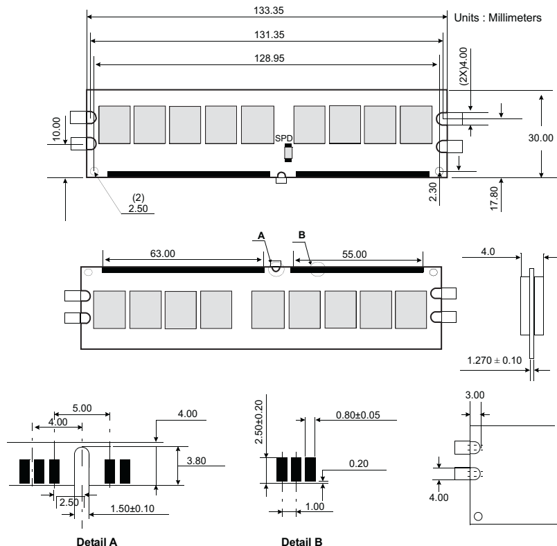
Figure 1: KVR533D2E4/1GI 240-Pin DIMM
