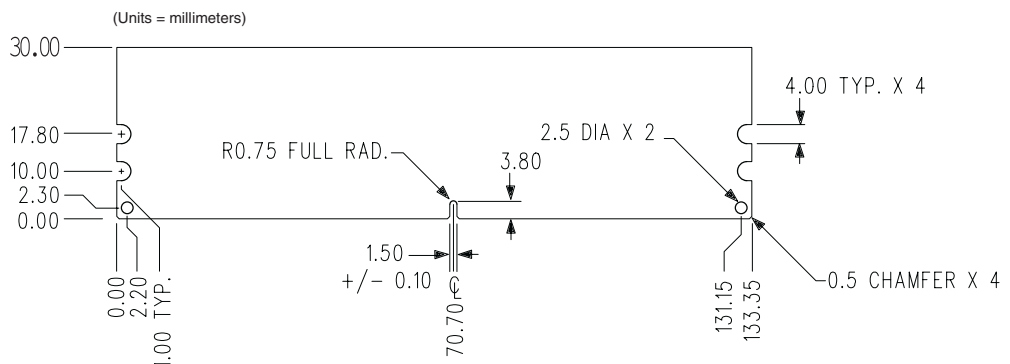
Figure 1: KVR400D2D4R3/4GI 240-Pin DIMM
