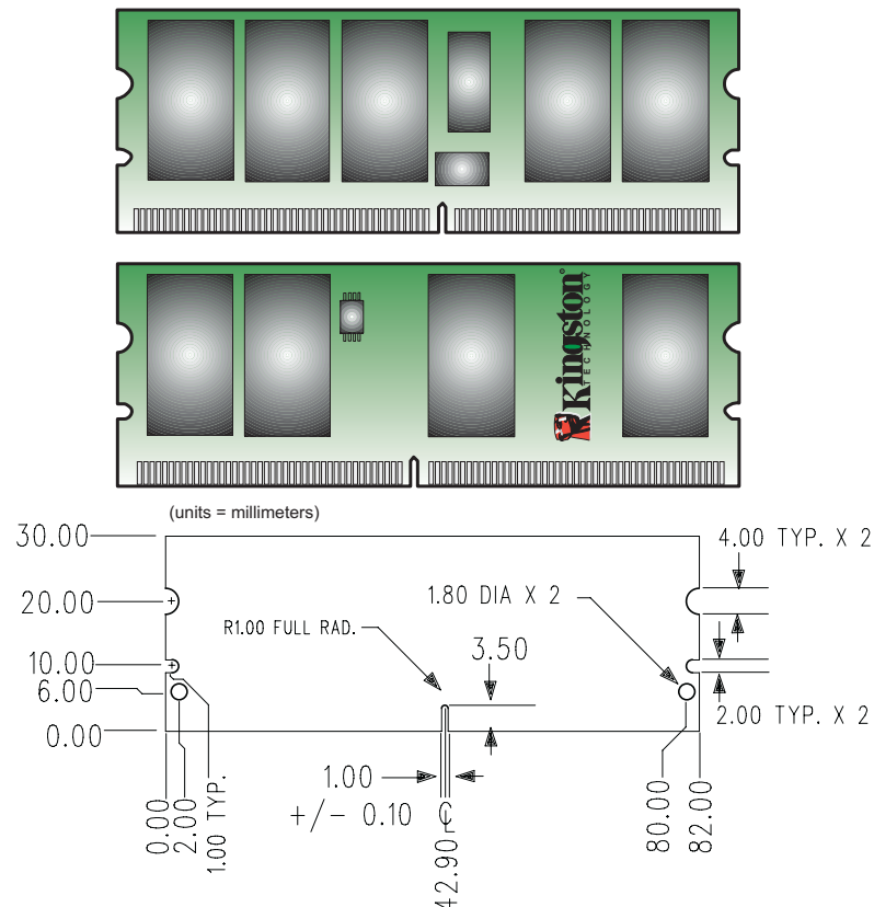
Figure 1: KVR533D2M4/512 244-Pin MiniDIMM
