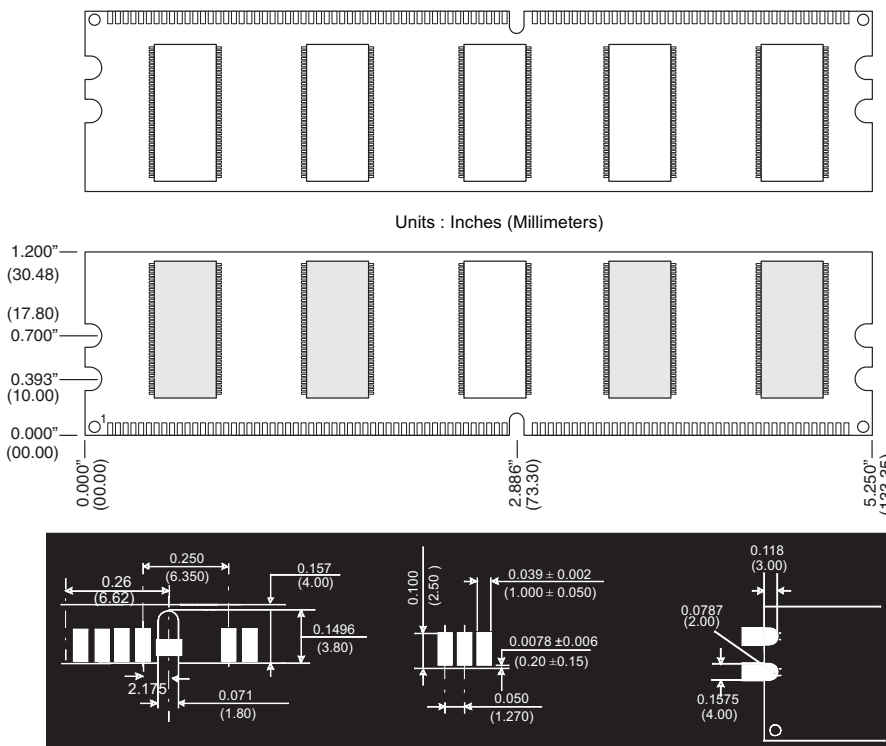
Figure 1: KVR400X64C3AK2/256 184-Pin DIMM
