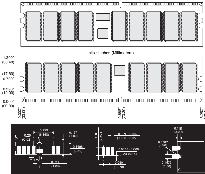
Figure 1: KVR266X72RC25L/2G 184-Pin DDR SDRAM Module
