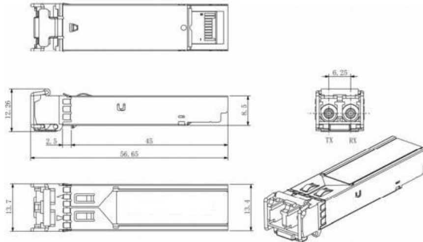
Mechanical Drawing
