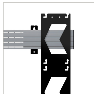
Interface arms feature directional arrows to indicate the panel install sequence, aiding a quick and easy installation
