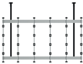
Ceiling Mount for INFILED WP Series 5x5 DVLED Videowall
