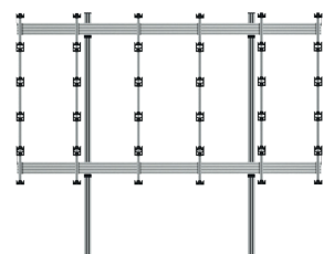
Bolt Down Stand for INFILED WP Series 5x5 DVLED Videowall
