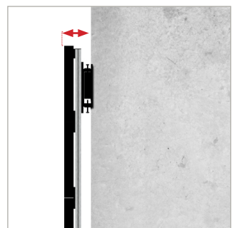
Close to the wall install - Only 121mm from the wall to the front of the panel
