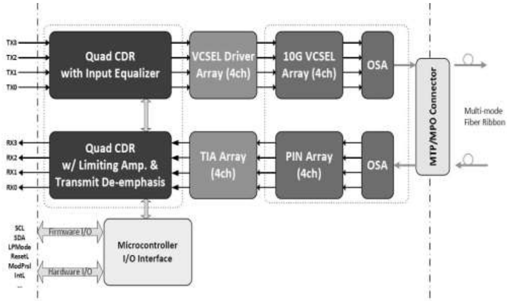
Figure1: Block Diagram
