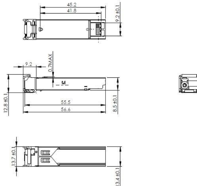
Mechanical Drawing
