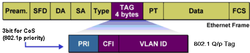
Figure 8-2 802.1Q frame
