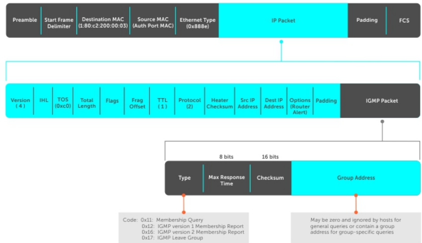
Figure 36. IGMP Messages in IP Packets
