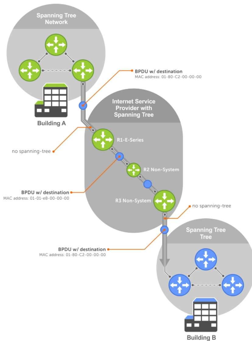
Figure 114. VLAN Stacking with L2PT
