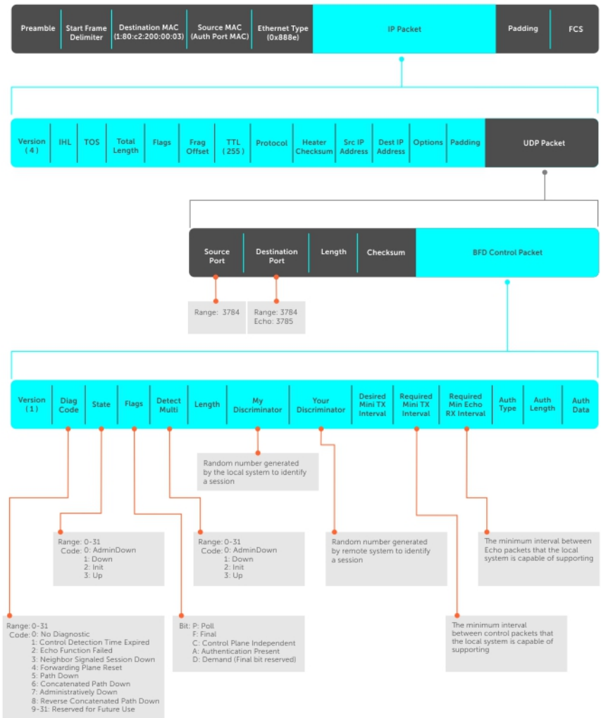
Figure 9. BFD in IPv4 Packet Format
