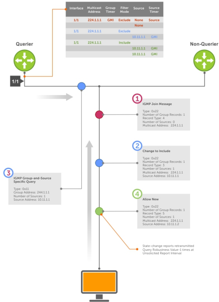
Figure 39. Membership Reports: Joining and Filtering
