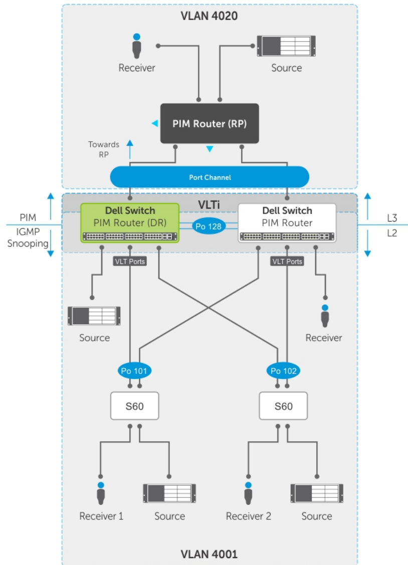
Figure 130. PIM-Sparse Mode Support on VLT
