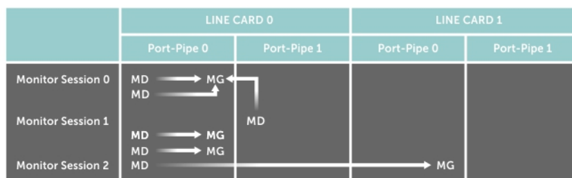
Figure 92. Port Monitoring Configurations
