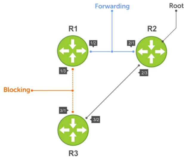
Figure 84. MSTP with Three VLANs Mapped to Two Spanning Tree Instances
