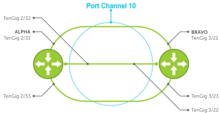
Figure 54. LACP Basic Configuration Example
