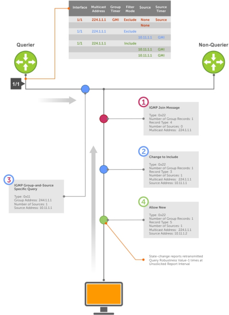
Figure 38. Membership Reports: Joining and Filtering
