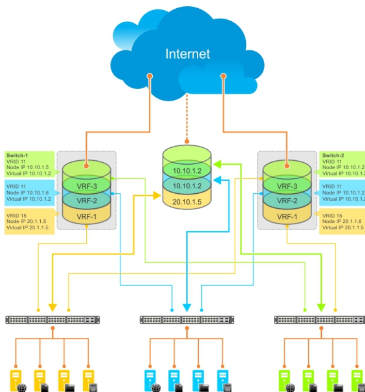
Figure 146. VRRP in a VRF: Non-VLAN Example
