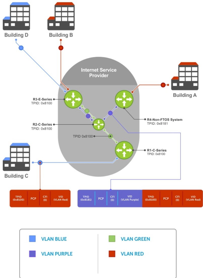
Figure 106. Single and Double-Tag TPID Match
