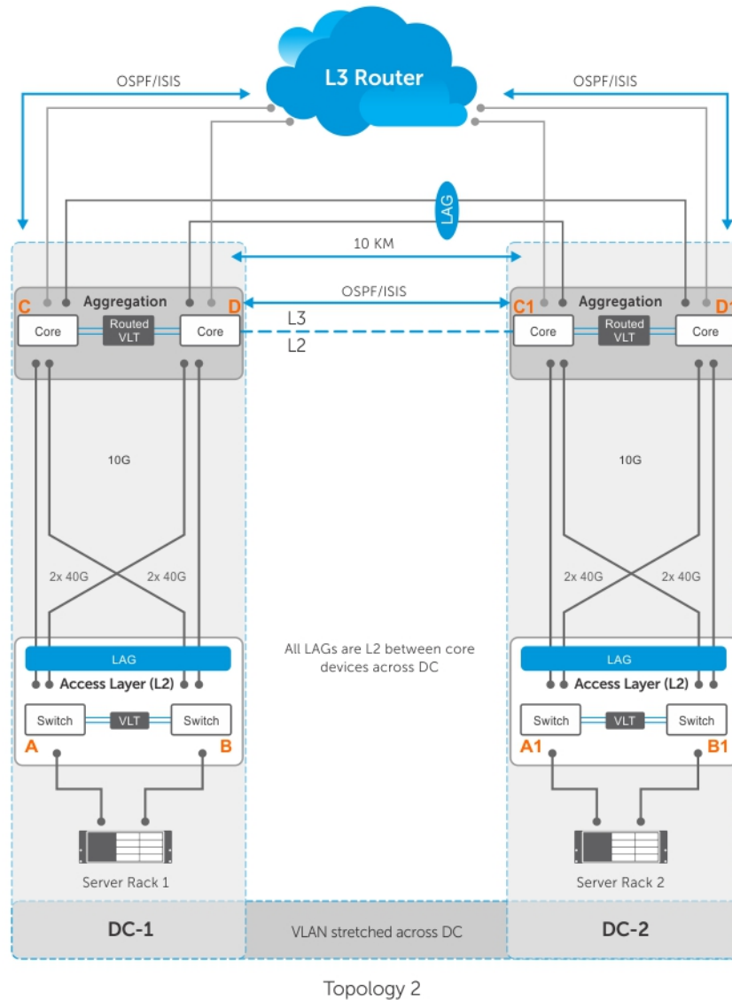
Figure 138. Sample Configuration for a VLT Proxy Gateway
