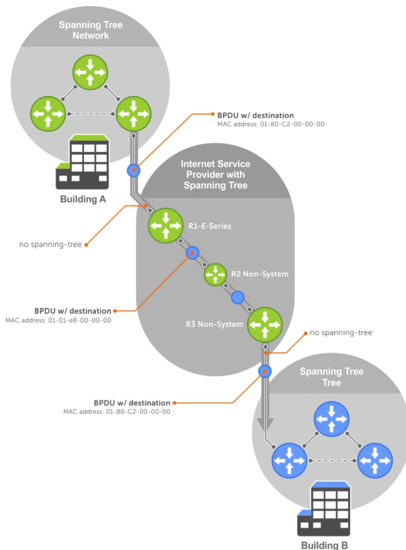
Figure 111. VLAN Stacking with L2PT
