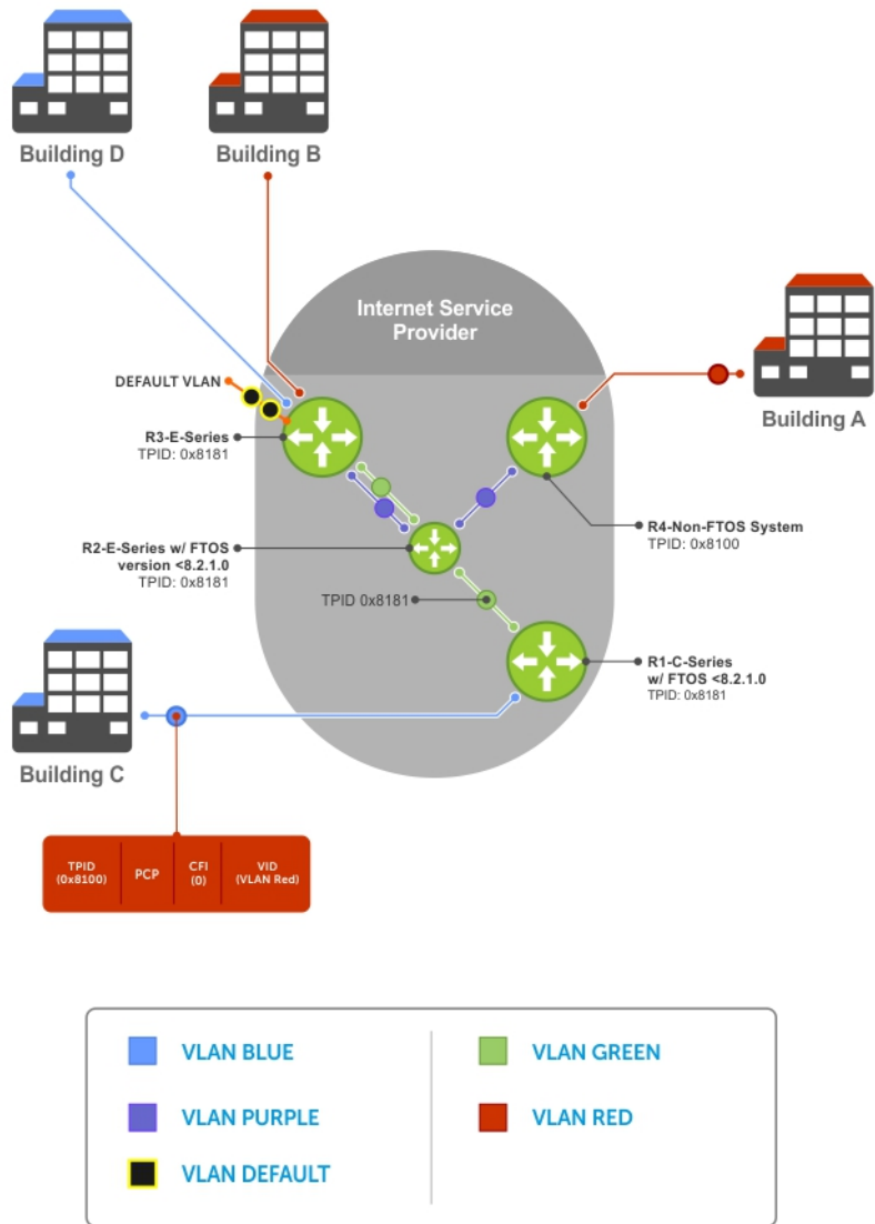
Figure 107. Single and Double-Tag First-byte TPID Match
