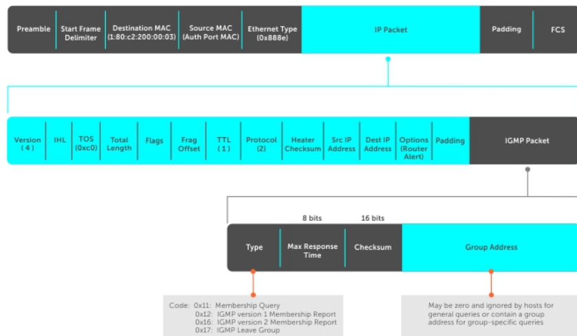
Figure 35. IGMP Messages in IP Packets
