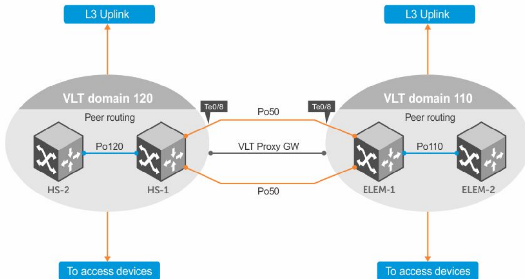
Figure 139. VLT Proxy Gateway Sample Topology
