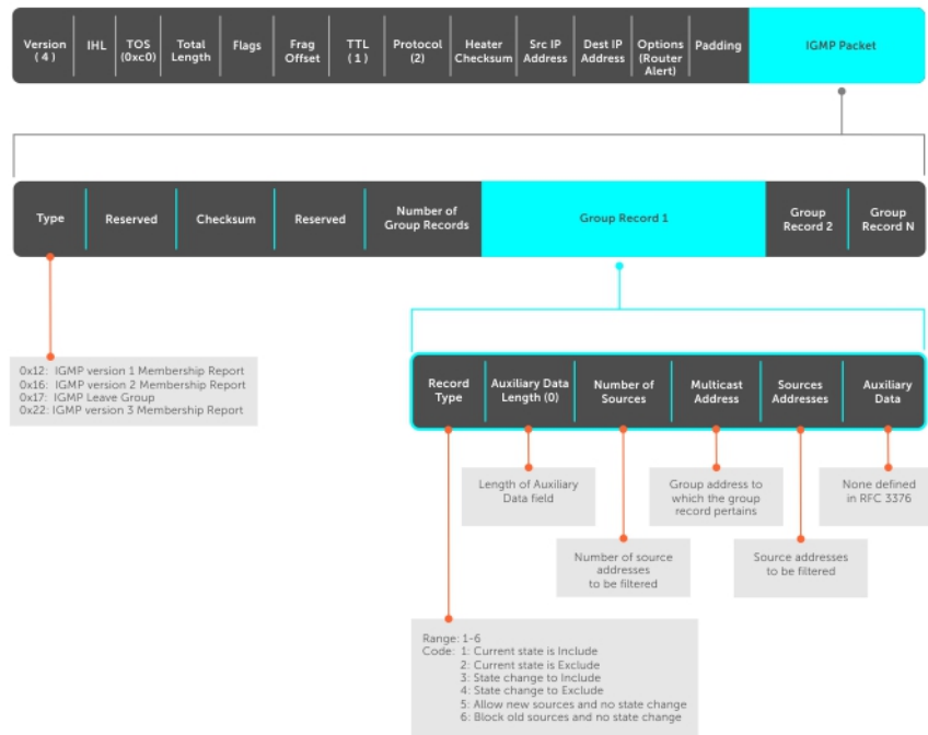
Figure 37. IGMP Version 3–Capable Multicast Routers Address Structure
