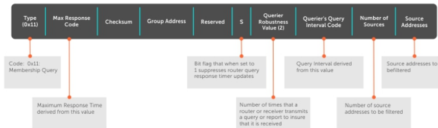
Figure 36. IGMP Version 3 Packet Structure
