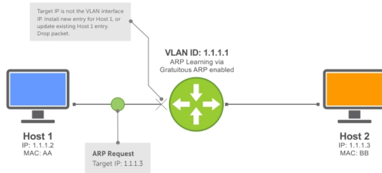
Figure 43. ARP Learning via ARP Request with ARP Learning via Gratuitous ARP Enabled
