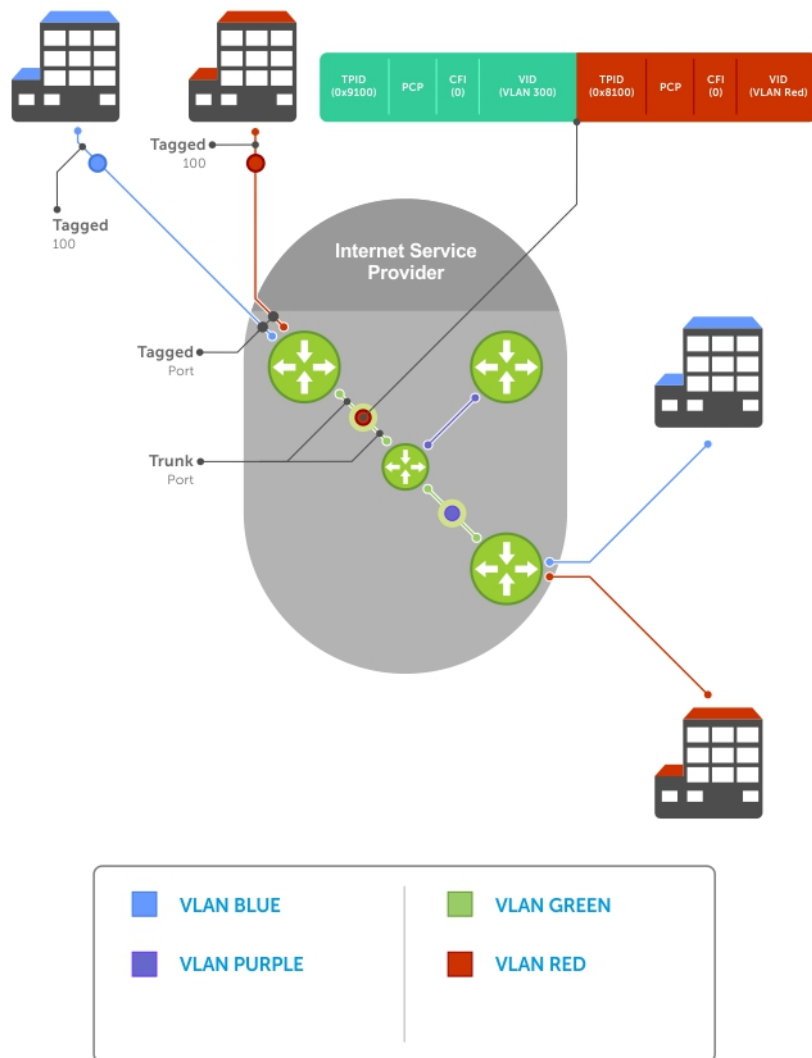
Figure 105. VLAN Stacking in a Service Provider Network
