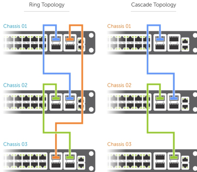
Figure 112. Supported Stacking Topologies
