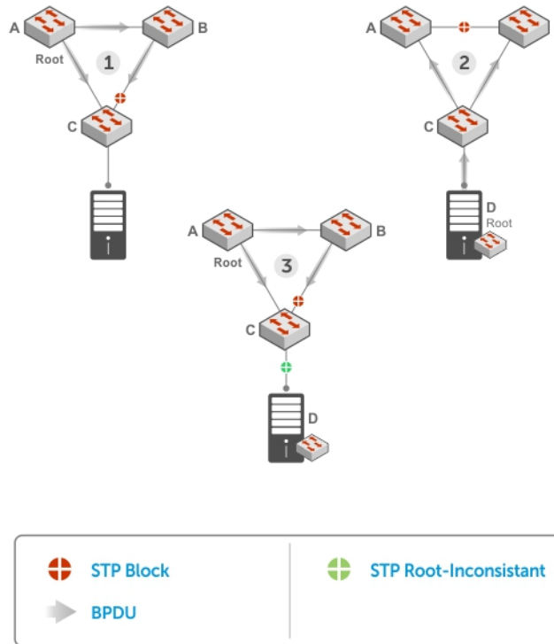
Figure 117. STP Root Guard Prevents Bridging Loops
