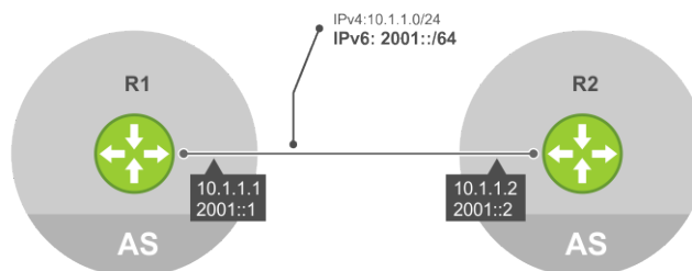
Figure 25. Configure IPv6 NH to advertise IPv6 prefix over IPv4 neighbor
