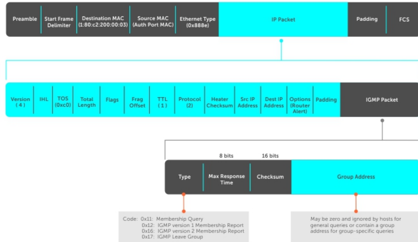
Figure 35. IGMP Messages in IP Packets
