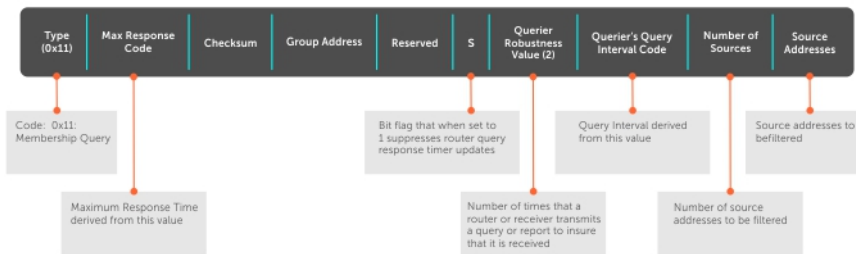
Figure 36. IGMP Version 3 Packet Structure
