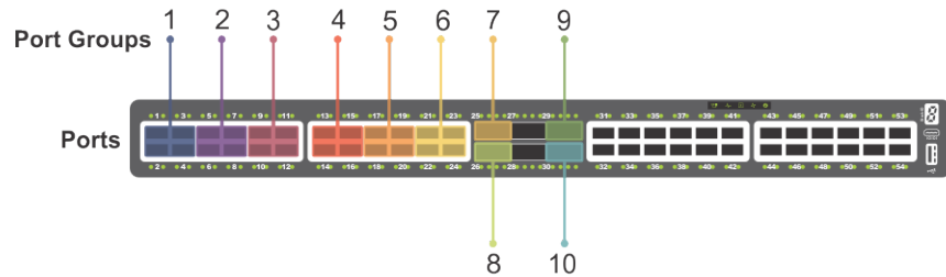
Figure 2. S4148U-ON unified port groups
