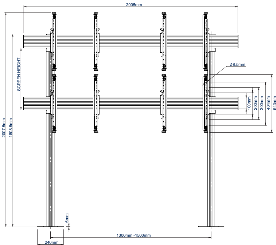
FRONT VIEW
