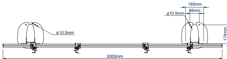
TOP VIEW
