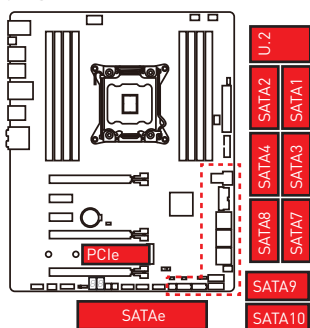
1 x M.2 PCIe + 1 x U.2 + 1 x SATAe + 8 x SATA *
