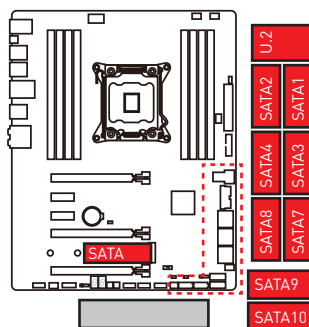
1 x M.2 SATA + 1 x U.2 + 8 x SATA
