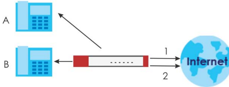
Figure 293 VoIP with Multiple WAN IP Addresses
