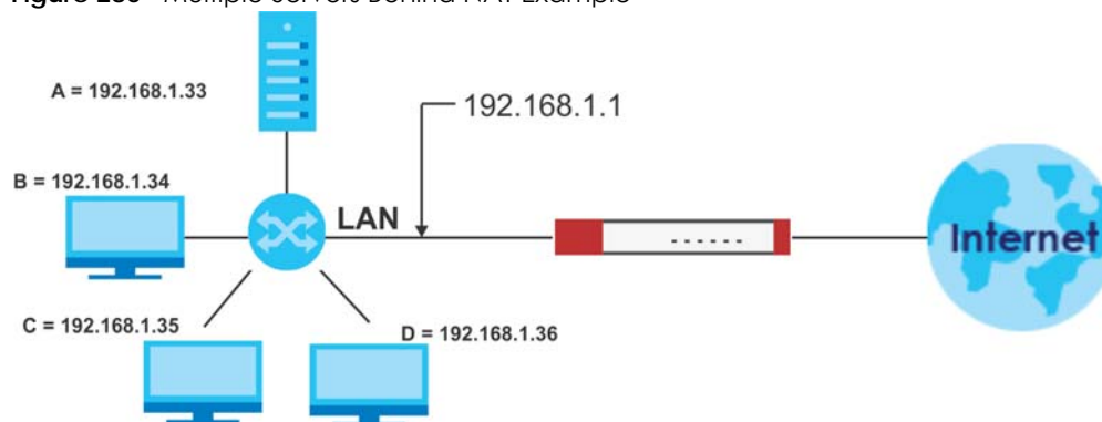
Figure 280 Multiple Servers Behind NAT Example
