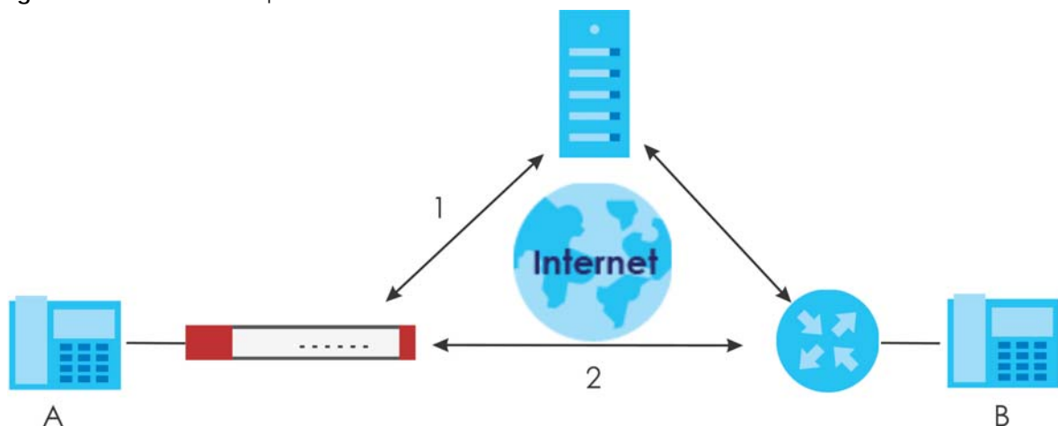
Figure 290 SIP ALG Example
