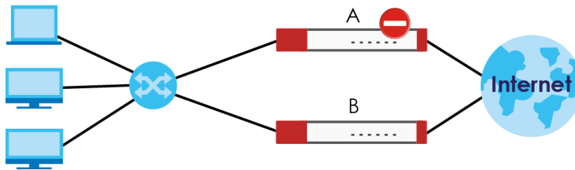
Figure 501 Device HA Backup Taking Over for the Master
