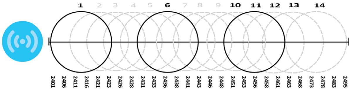
Figure 221 An Example Three-Channel Deployment
