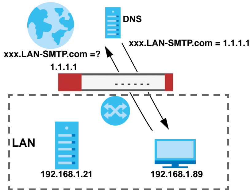
Figure 283 LAN Computer Queries a Public DNS Server
