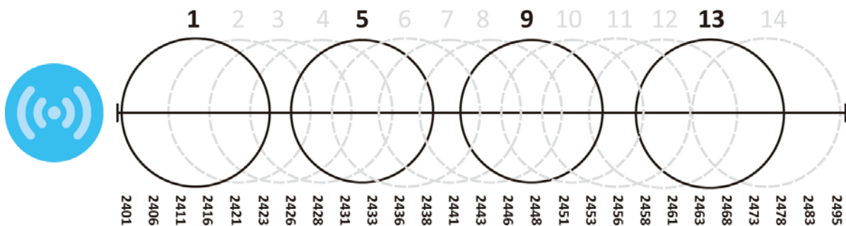
Figure 223 An Alternative Four-Channel Deployment
