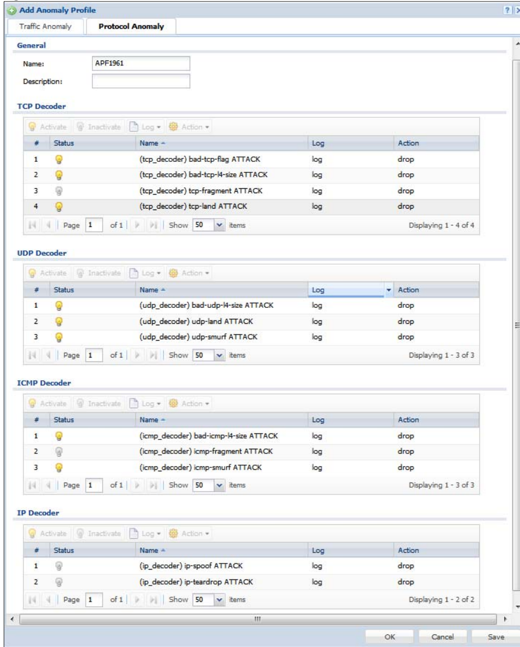
Figure 379 Configuration > Security Policy > ADP > Profile > Add-Protocol-Anomaly
