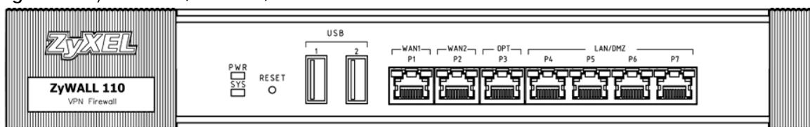
Figure 40 ZyWALL 310 / ZyWALL 1100 / USG310 / USG1100 / USG1900 Front Panel
