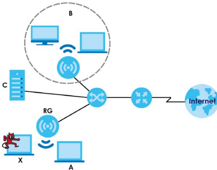
Figure 535 Rogue AP Example
