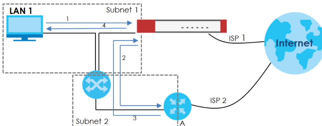
Figure 373 Using Virtual Interfaces to Avoid Asymmetrical Routes
