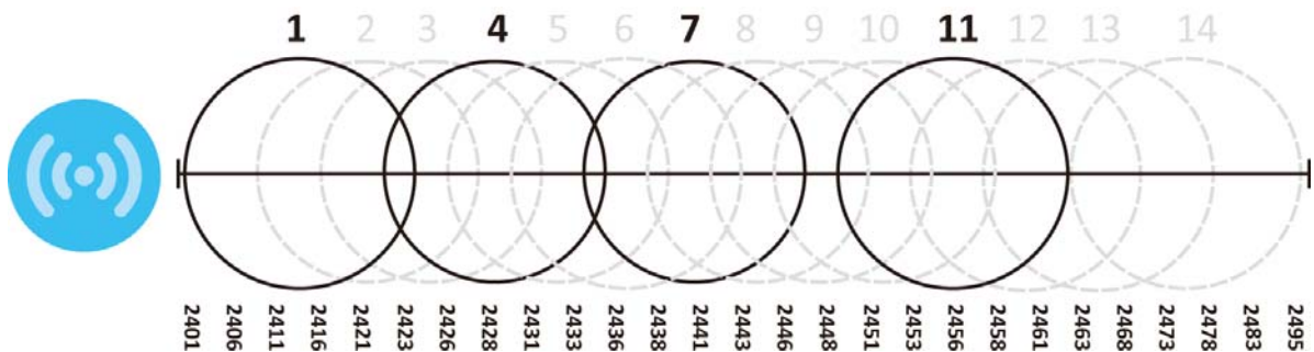
Figure 222 An Example Four-Channel Deployment
