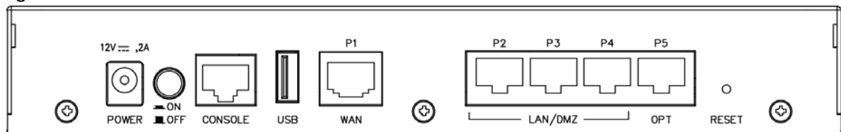
Figure 50 USG40 / USG40W Rear Panel
