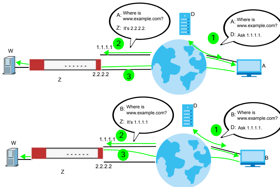
Figure 314 DNS Load Balancing Example
