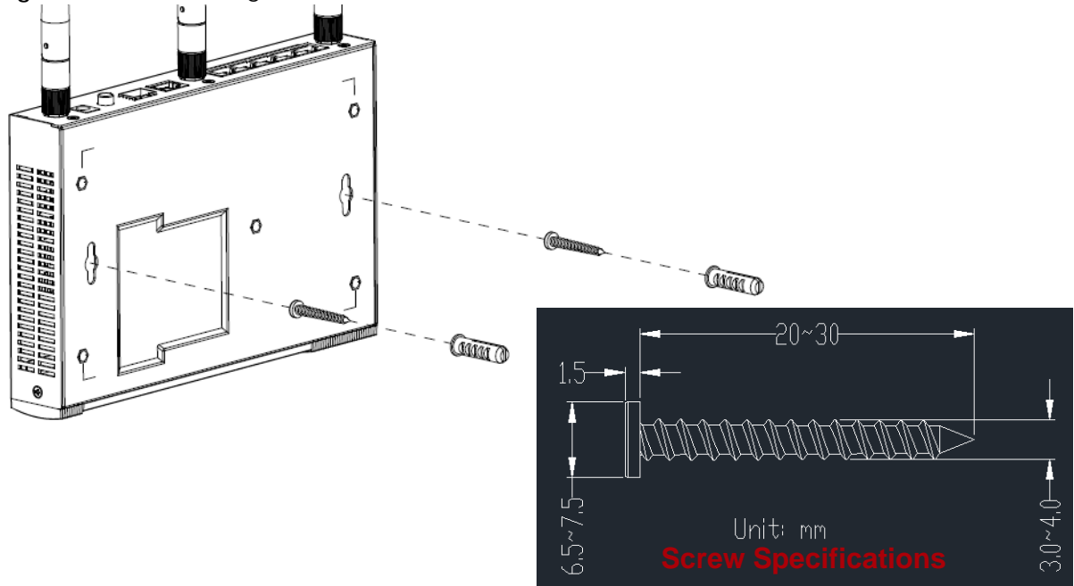
Figure 54 Wall Mounting
