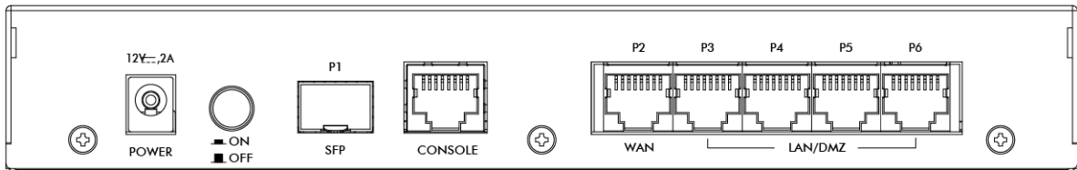
Figure 52 USG60 / USG60W Rear Panel
