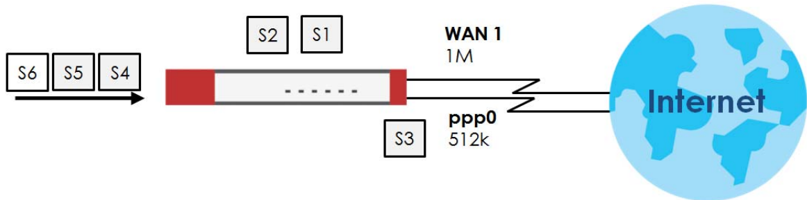
Figure 257 Weighted Round Robin Algorithm Example
