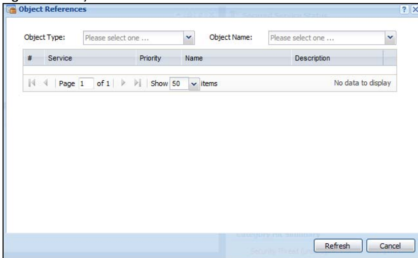
Figure 12 Object Reference
