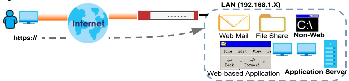
Figure 390 SSL VPN
