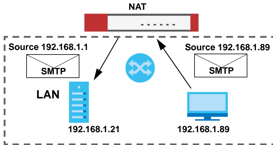
Figure 284 LAN to LAN Traffic
