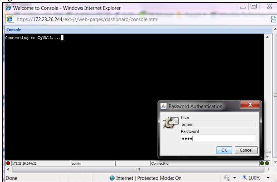
Figure 13 Console Window
