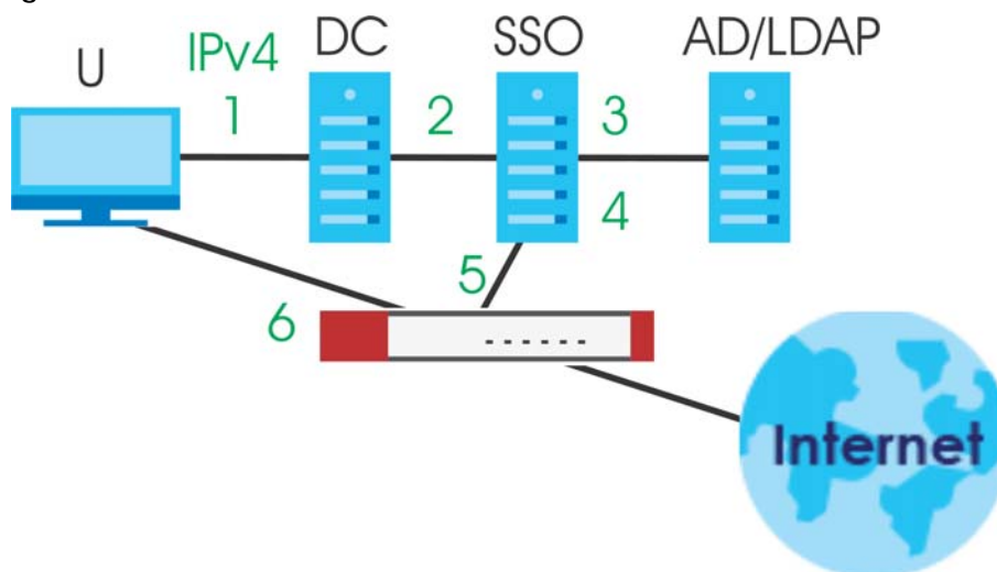
Figure 336 SSO Overview
