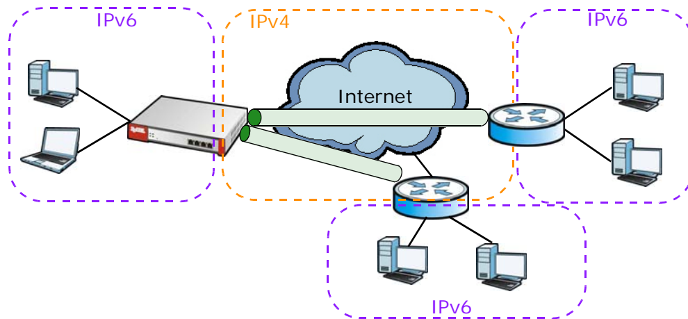
Figure 242 6to4 Tunnel
