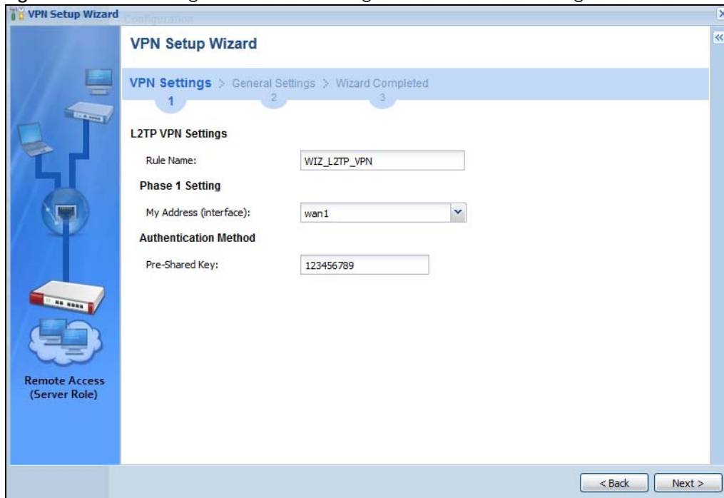
Figure 142 VPN Settings for L2TP VPN Settings Wizard: L2TP VPN Settings
