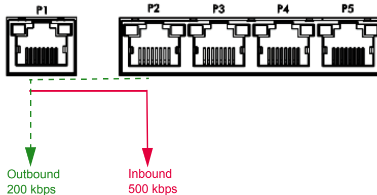
Figure 450 LAN1 to WAN, Outbound 200 kbps, Inbound 500 kbps
