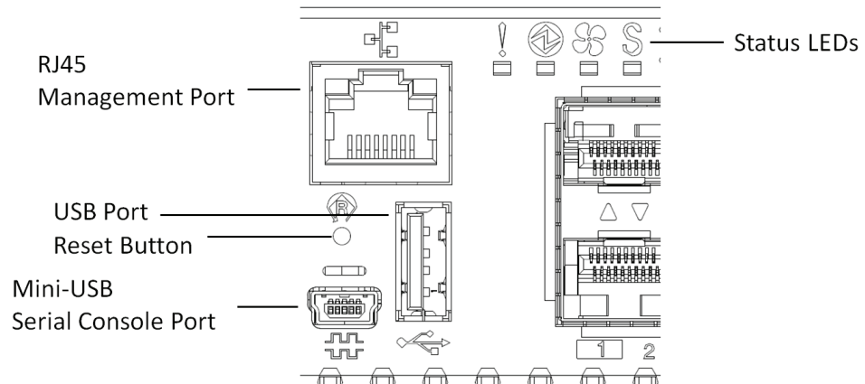
Figure 3. NE1032 rear panel
