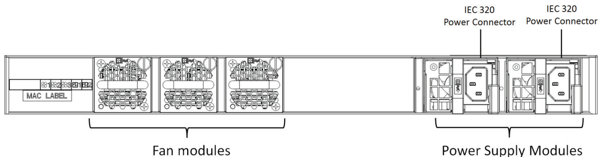
Figure 3. NE1032 rear panel
