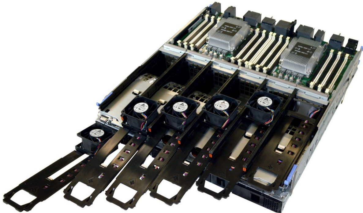
Figure 18. Six fans installed in each compute tray (lower compute tray shown)
