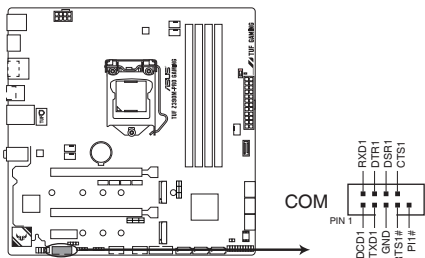
TUF Z390M-PRO GAMING Serial port connector
