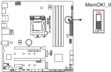
TUF Z390M-PRO GAMING MemOK! switch
