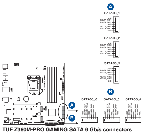
TUF Z390M-PRO GAMING SATA 6 Gb/s connectors
