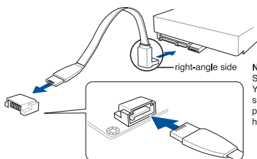
TUF Z390M-PRO GAMING SATA 6 Gb/s connectors
