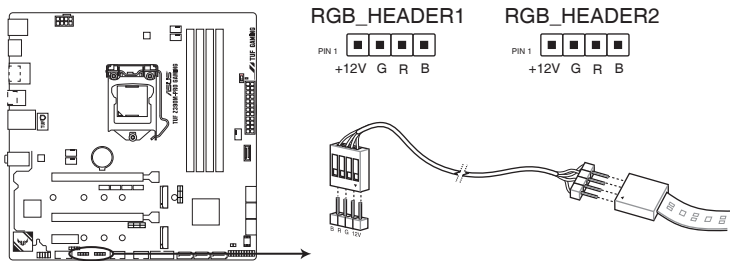
TUF Z390M-PRO GAMING RGB_HEADER connectors
