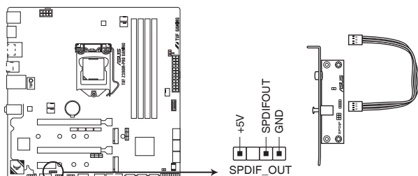
TUF Z390M-PRO GAMING Digital audio connector
