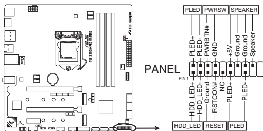
TUF Z390M-PRO GAMING System panel connector
