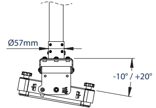
SIDE VIEW WITH INTERFACE TILT
