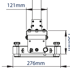
SIDE VIEW WITH CEILING PLATE TILT
