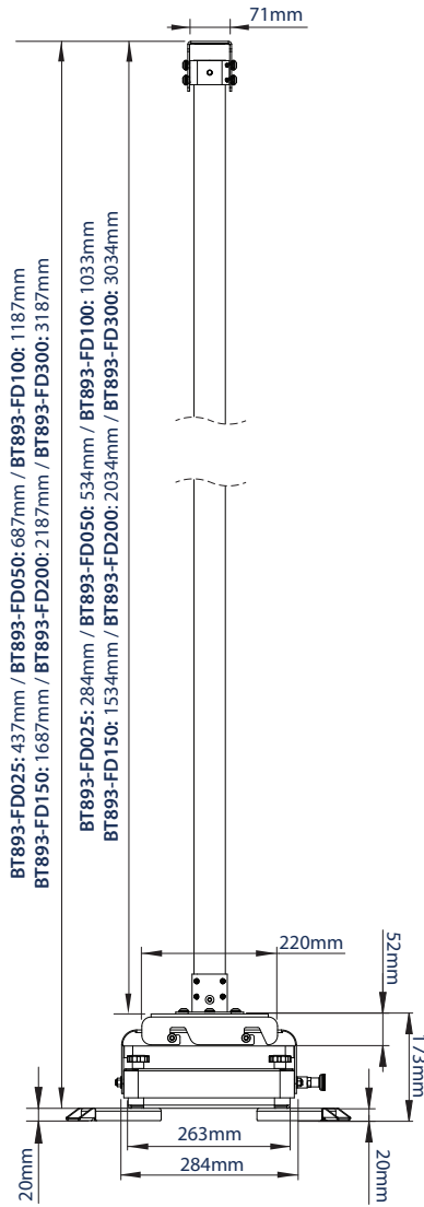
FRONT VIEW
