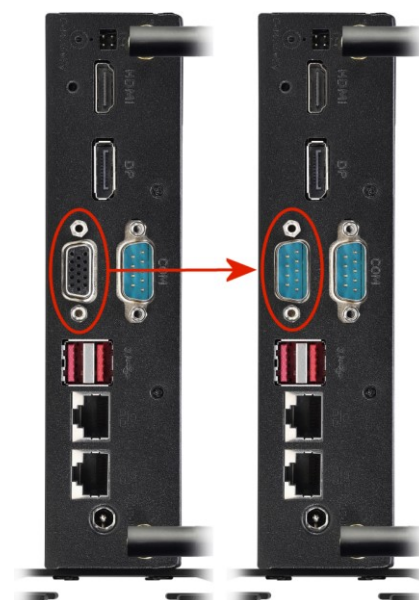
Shuttle XPC slim DS10U before and after the installation of one PCP11 adapter
