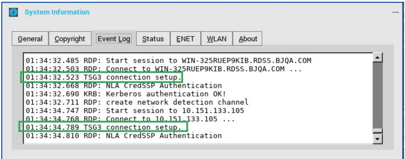
Figure 24. Event log tab
