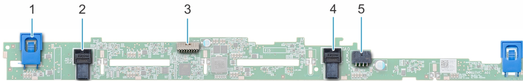
Figure 61. Backplane SAS/SATA/SSD de 2,5 pouces (x8)
