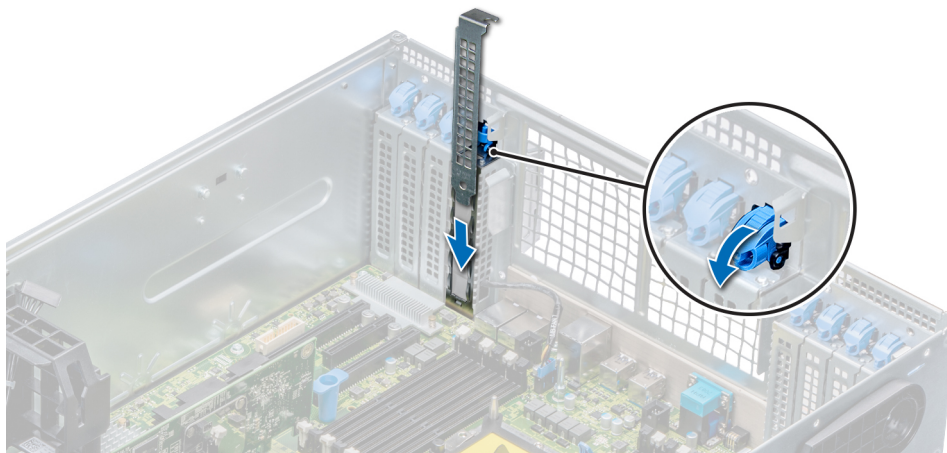
Figure 82. Installation de la plaque de recouvrement
