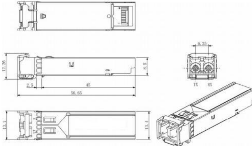
Mechanical Drawing
