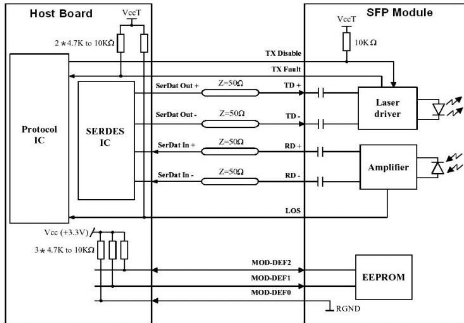
SFP Host Recommended Circuit
