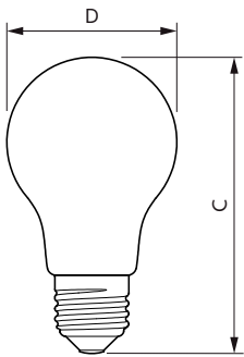
Bulb A67 100W 1521lm 2700K E27 NDFrosted
