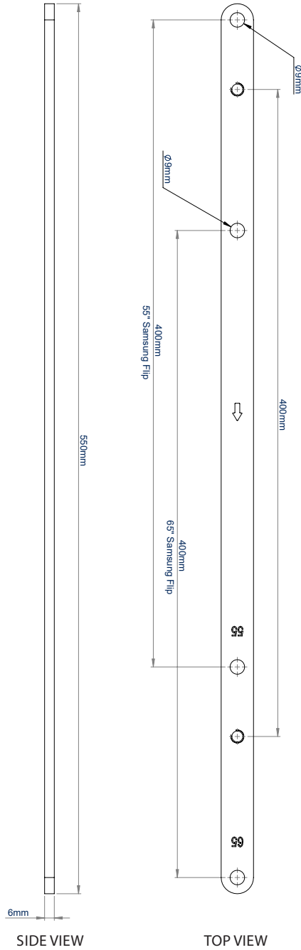
SIDE VIEW
