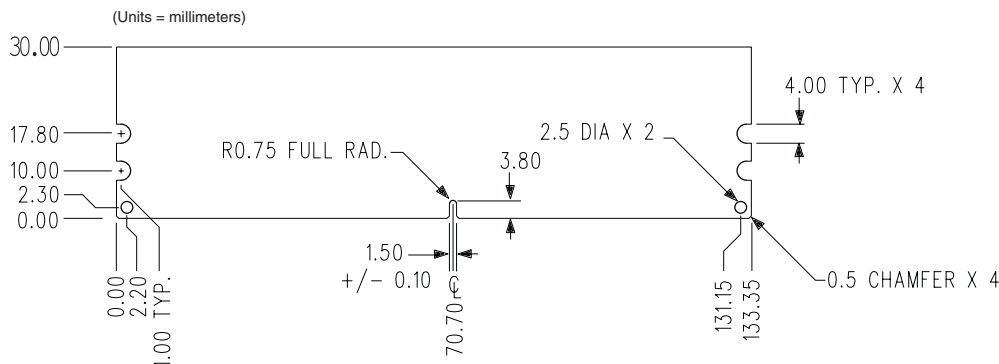
Figure 1: KVR800D2S8P6K2/2G 240-Pin DIMM
