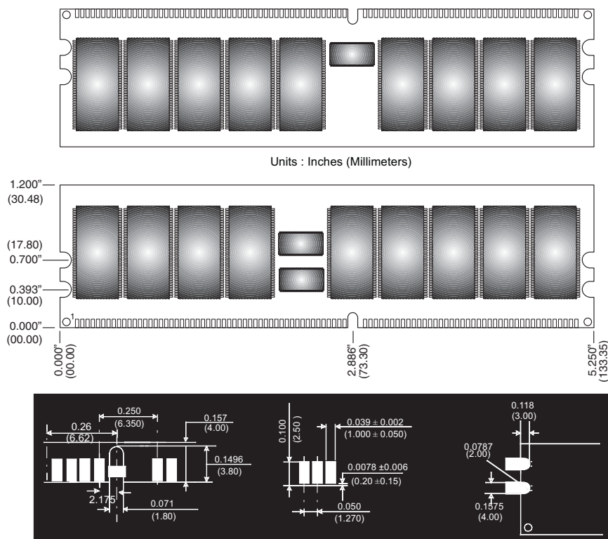
Figure 1: KVR266X72RC25L/512D 184-Pin DIMM
