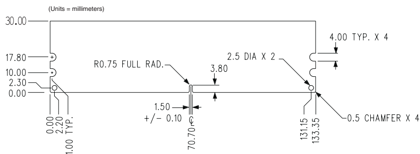
Figure 1: KVR667D2D8P5/2GEF 240-Pin DIMM
