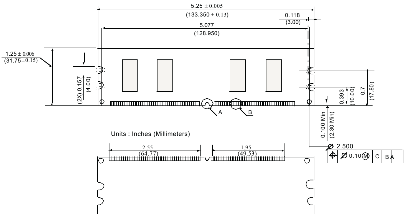
Figure 1: KVR400X64C3A/128 184-Pin DIMM
