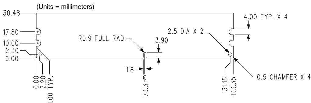
Figure 1: KVR400X72RC3A/2G 184-Pin DIMM
